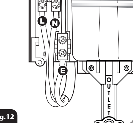
Terminal block
